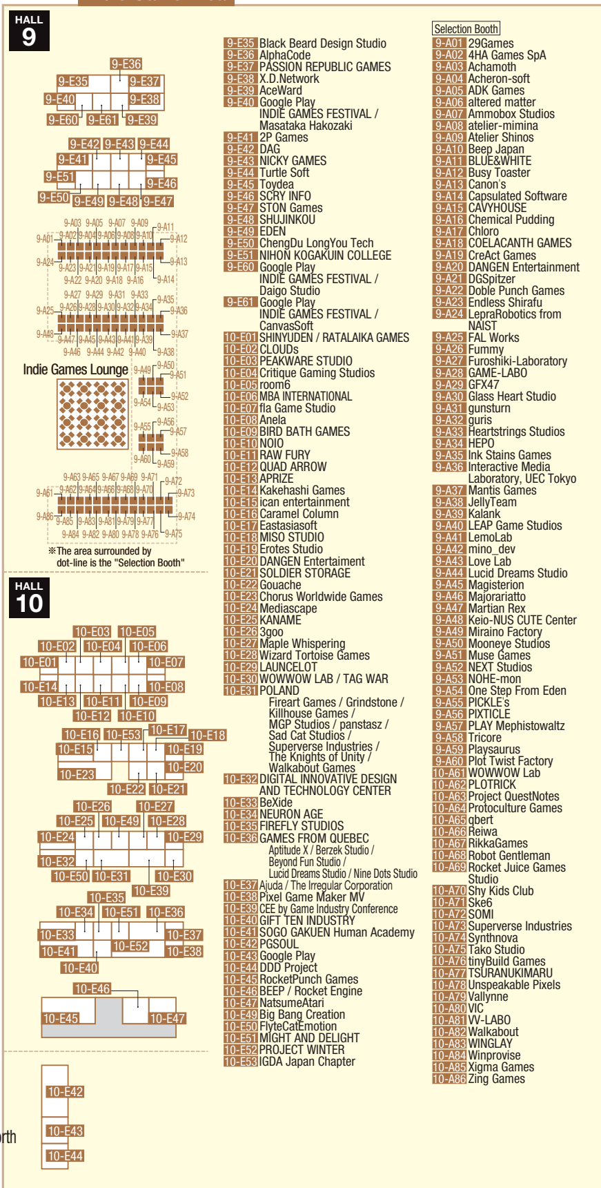
figure D New Stars Area
