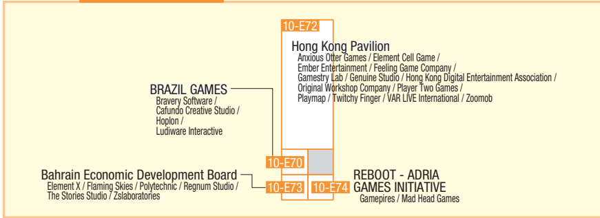
figure D New Stars Area
