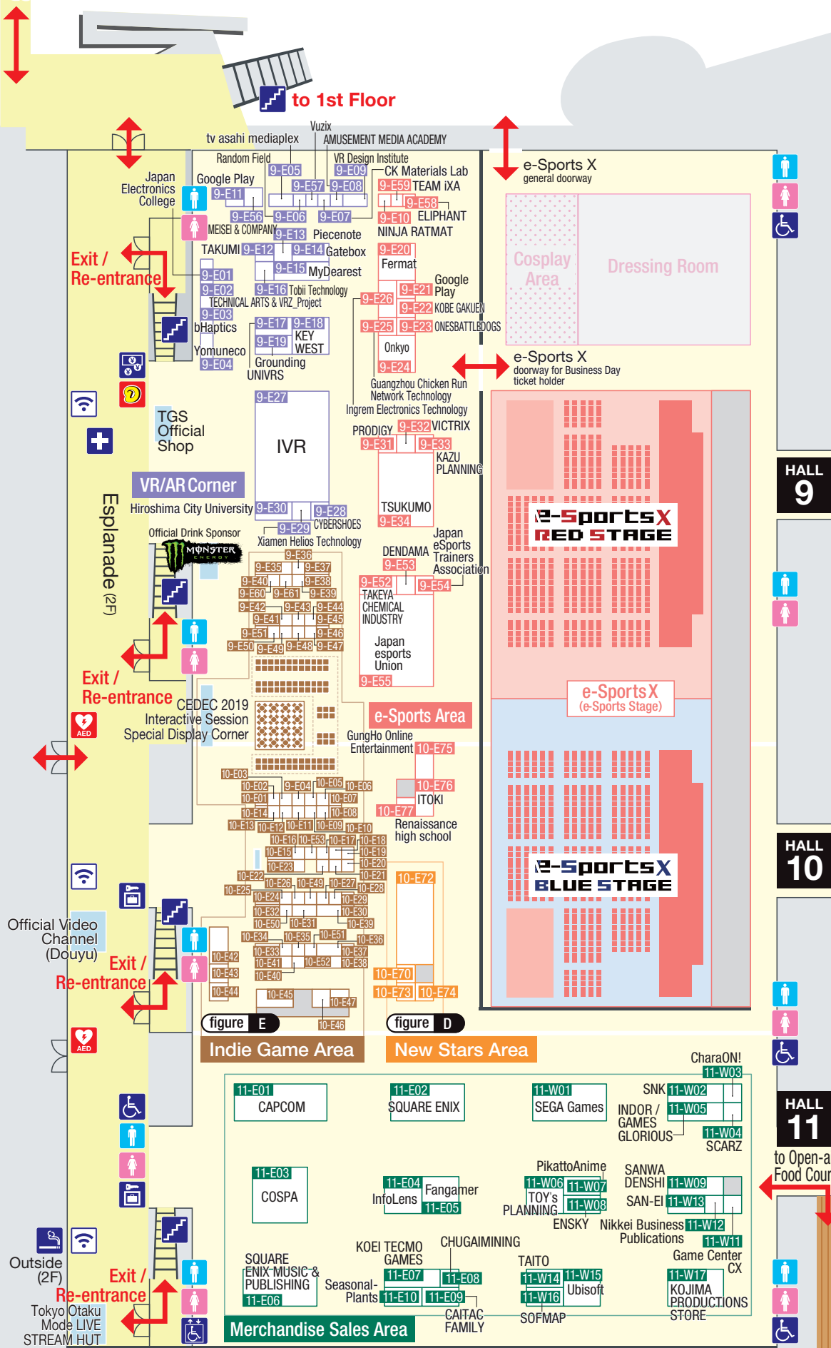
figure D New Stars Area
